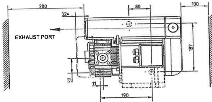
SPACE FOR EXHAUST FILTER EXCHANGE AND COOLING
